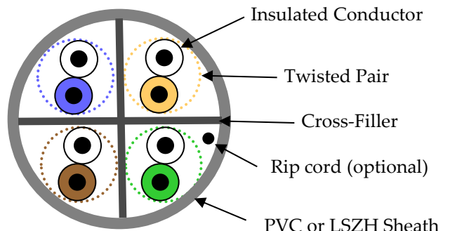
Fig 1. CrossSectional Diagram of Cable
